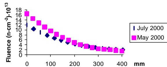
Figure 1: Neutron Flux distribution
