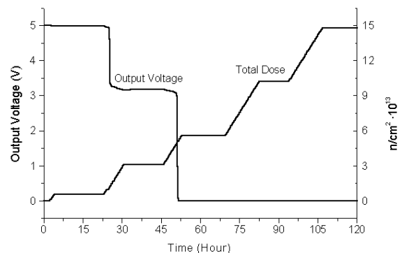
Figure 15: REF02 output Voltage & total dose
