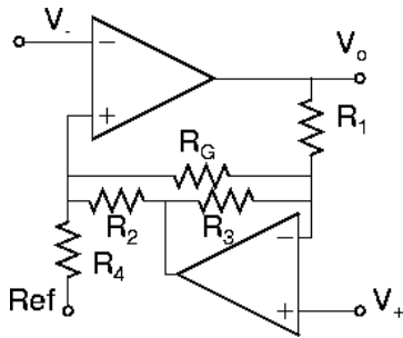
Figure 3: Two OpAmps I. Amplifier
