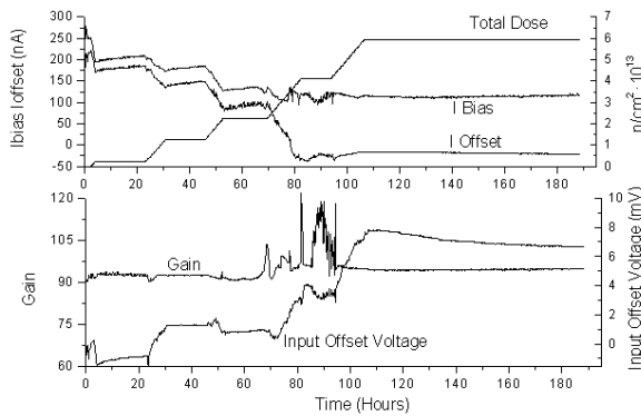
Figure 7: Three TLE2071 Instrumentation Amplifier
