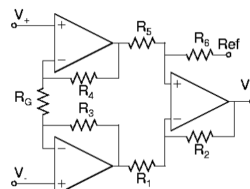
Figure 2: Three OpAmps I. Amplifier
